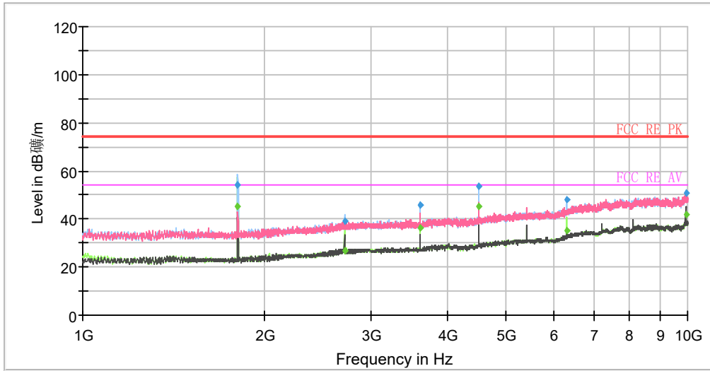
Radiates Emission from 1GHz to 10GHz
