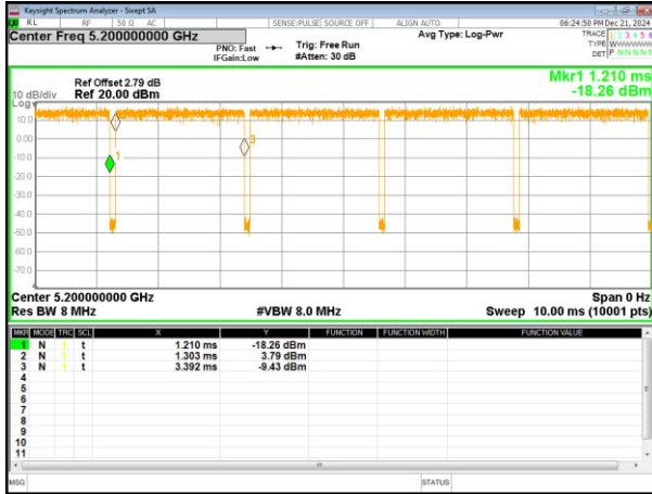
(802.11ac20) plot
