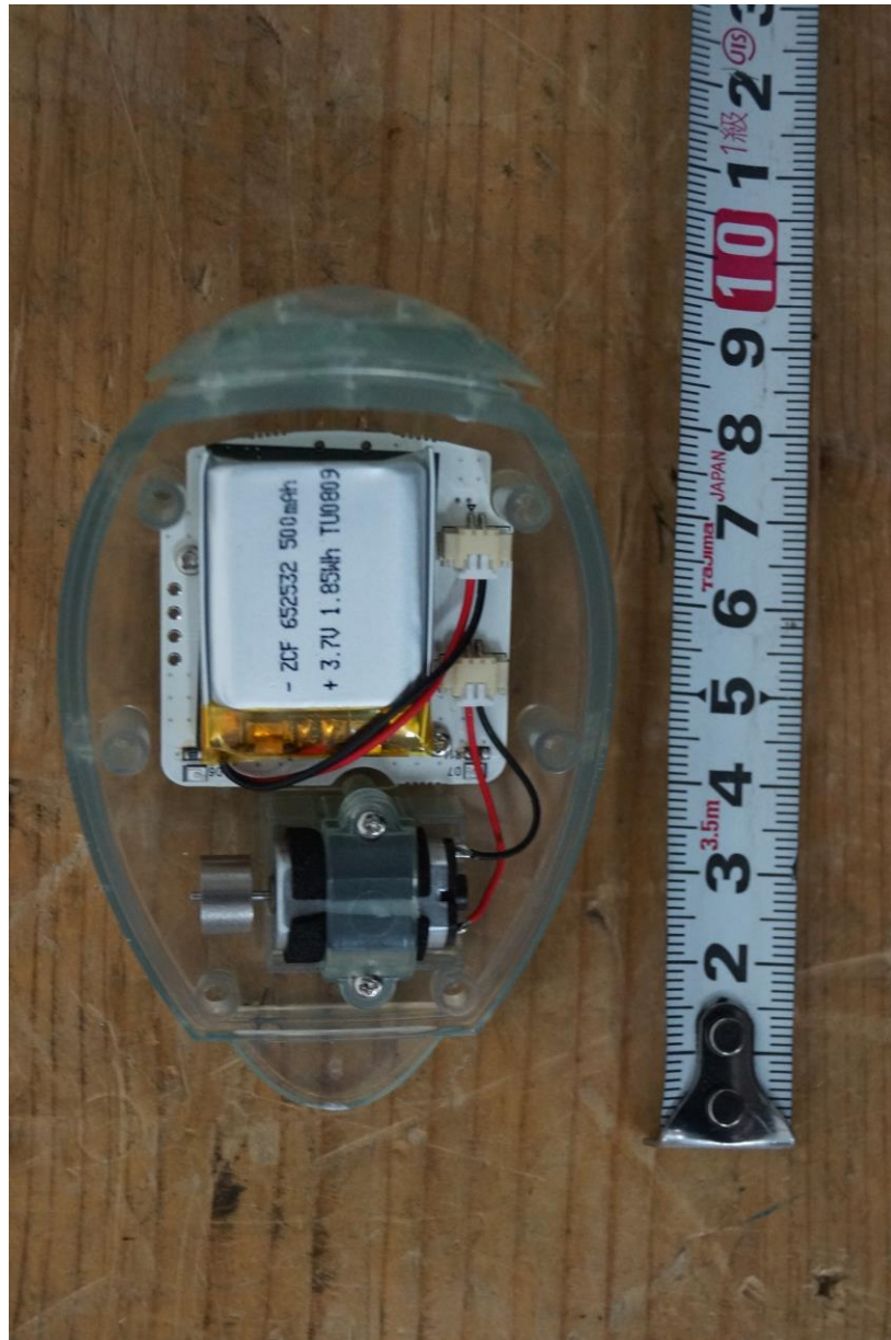
< Cleanser Inside view >
