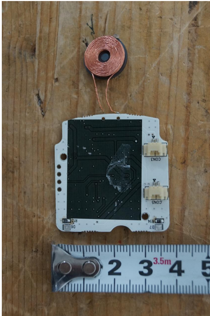
< Cleanser Main board bottom view >
