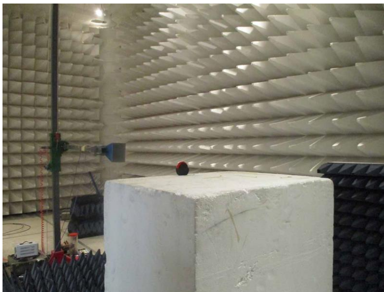
12GHz – 18GHz, Back View
