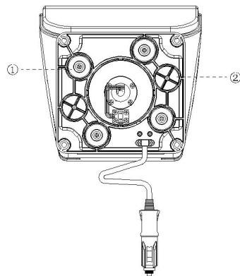
① — Comes with Magnetic ② — Magnet Installation Position
