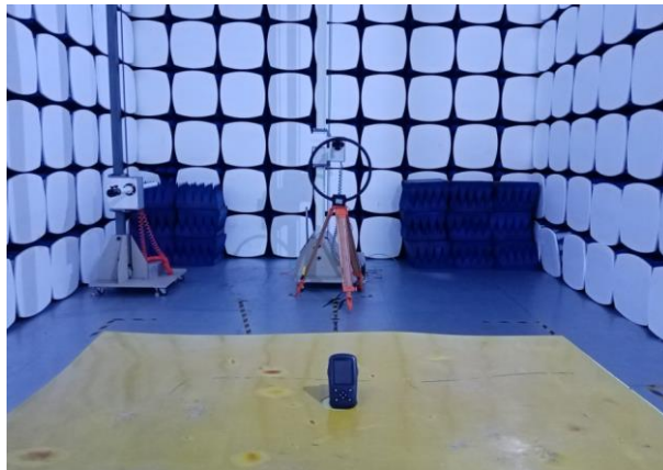
Radiated emission Below 30MHz
