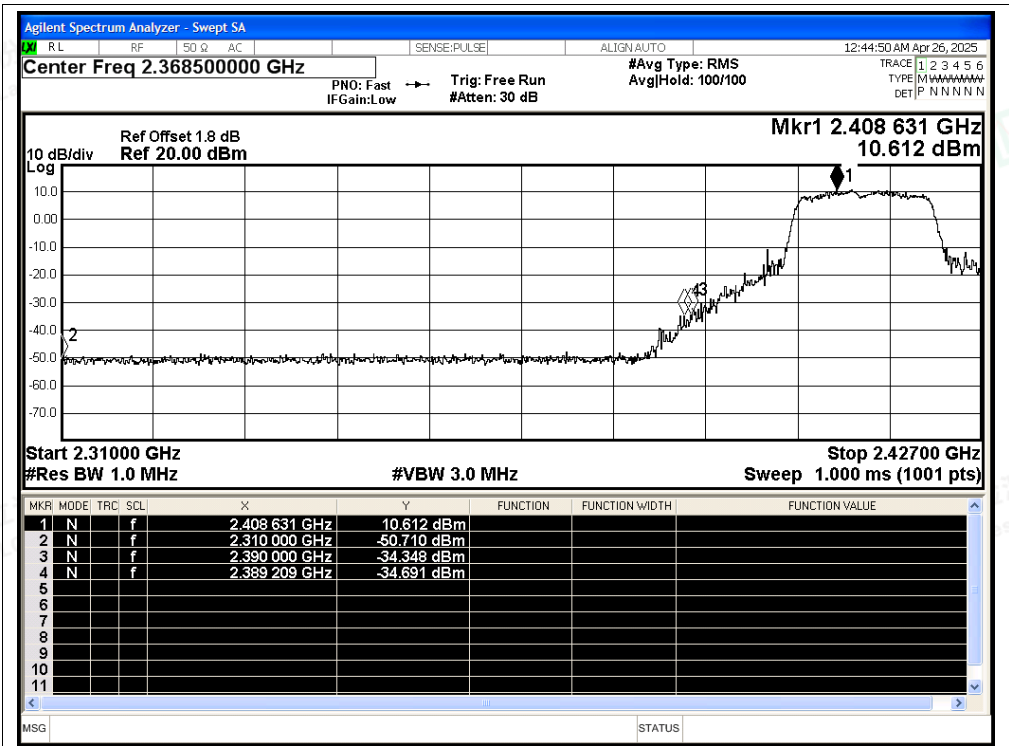
Restrict Band NVNT ax20 2412MHz Ant1 Average
