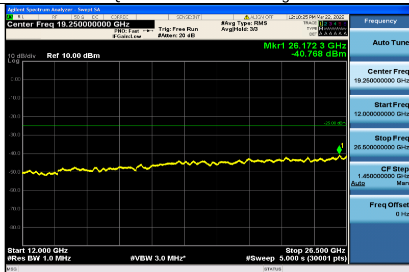
Band41-15MHz-16QAM-41165-75RB#0-Range4:12000~26500MHz
