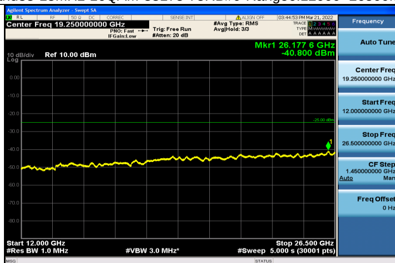
Band38-15MHz-16QAM-38175-75RB#0-Range6:12000~26500MHz
