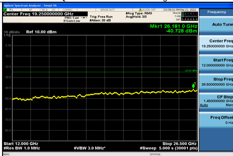
Band38-20MHz-16QAM-38150-100RB#0-Range6:12000~26500MHz
