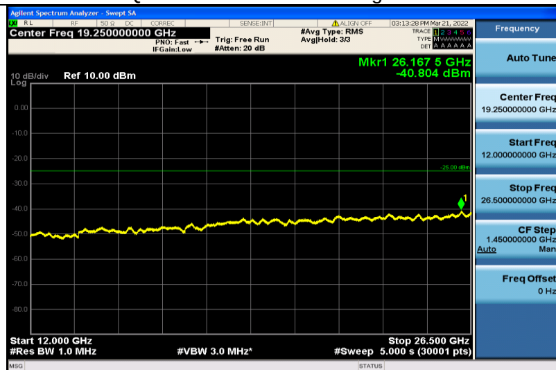
Band38-5MHz-QPSK-38000-25RB#0-Range6:12000~26500MHz
