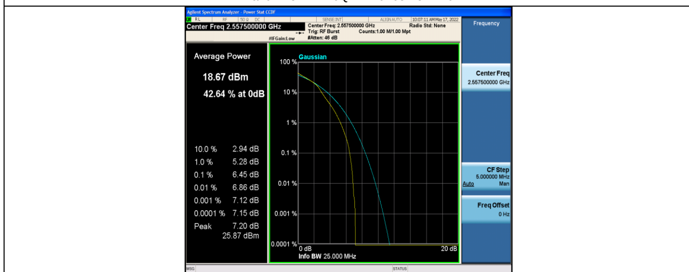
Band41-5MHz-16QAM-40740-1RB#0
