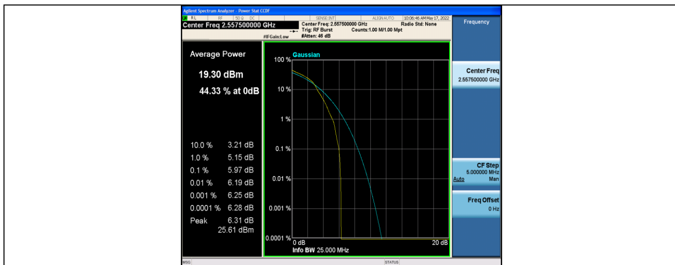
Band41-5MHz-16QAM-40265-25RB#0
