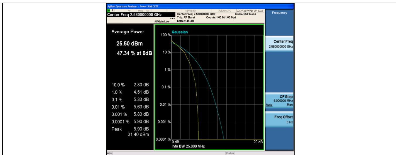
Band38-20MHz-QPSK-37850-100RB#0
