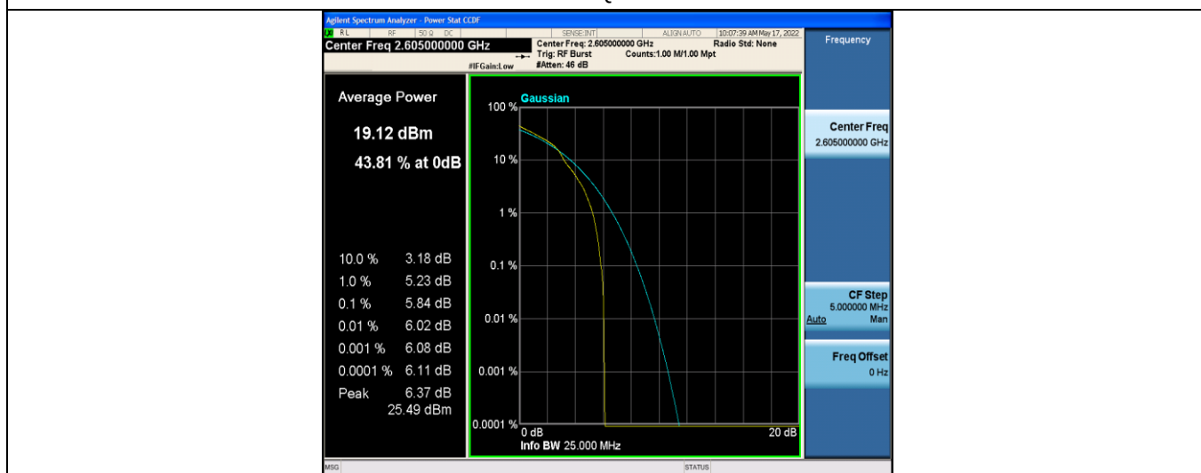
Band41-5MHz-16QAM-40740-25RB#0
