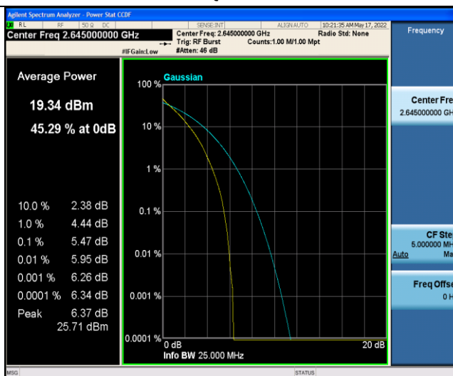
Band41-20MHz-16QAM-40340-1RB#0
