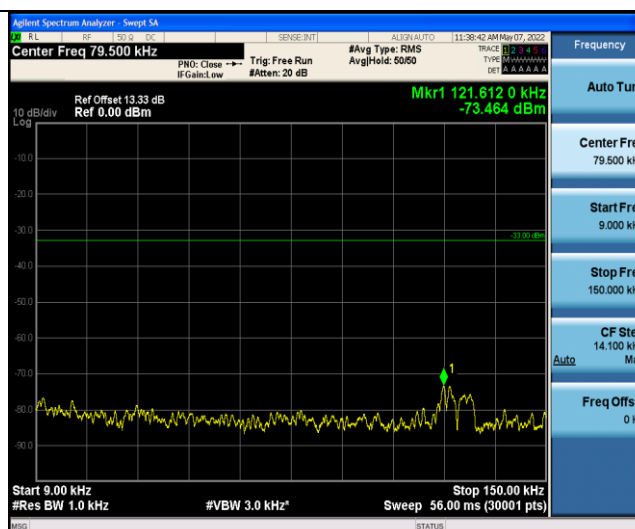
Band5-4183-2-10000~18000MHz
