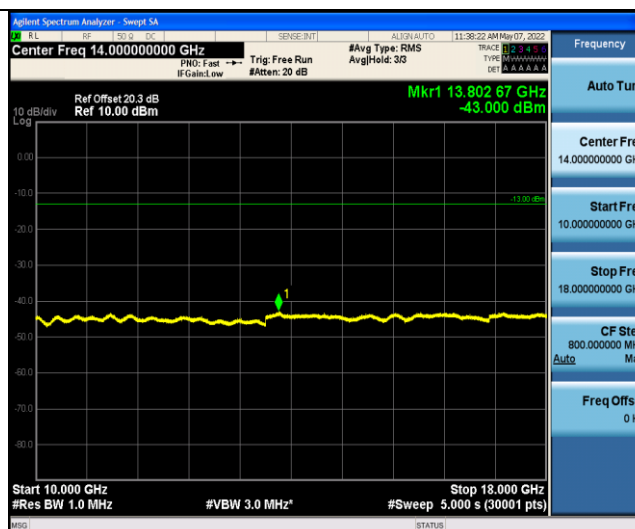
Band5-4132-3-10000~18000MHz
