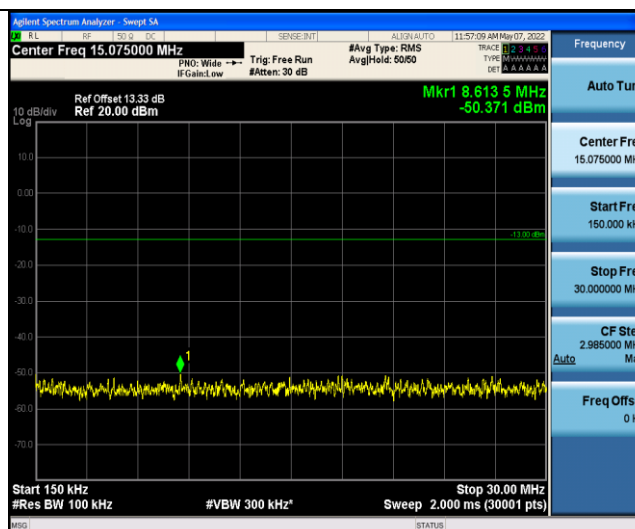
Band5-4183-1-0.15~30MHz
