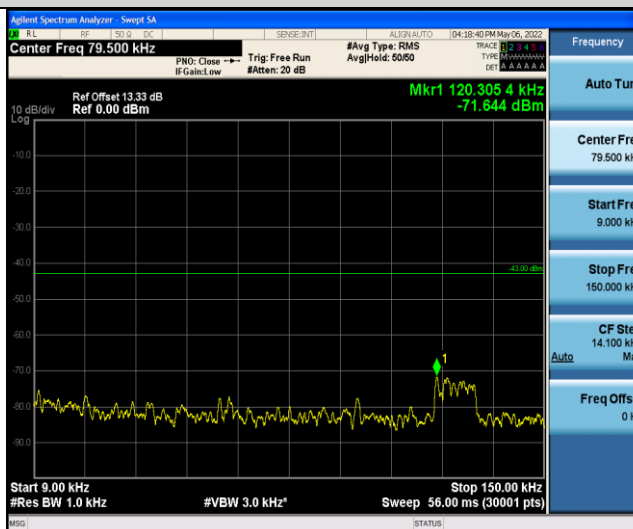
Band2-9538-1-0.009~0.15MHz
