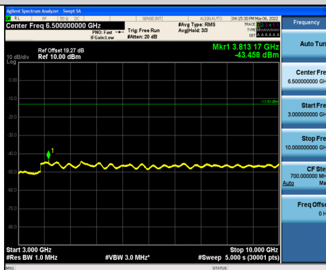
Band2-9538-4-3000~10000MHz
