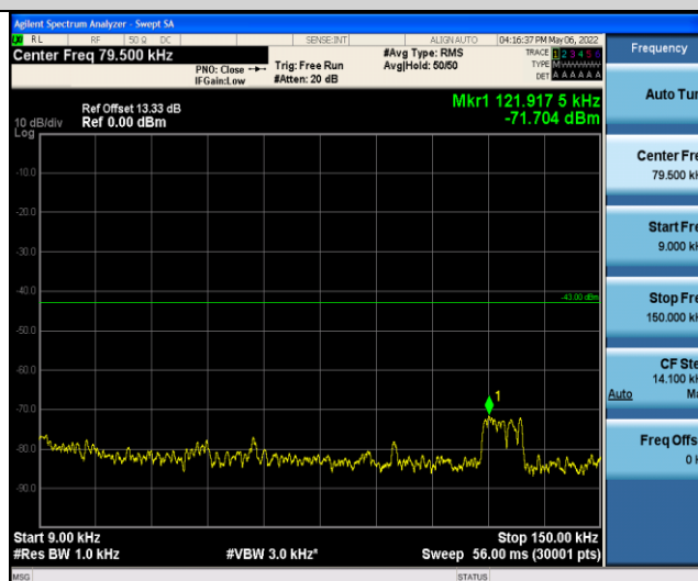
Band2-9400-1-0.009~0.15MHz
