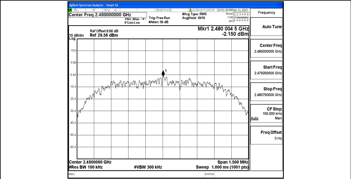
3DH5_Ant1_2480_30~1000
