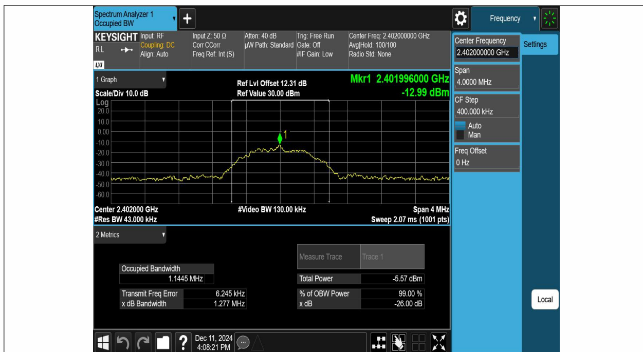
2.4G DTS MIMO-Ant2-2402
