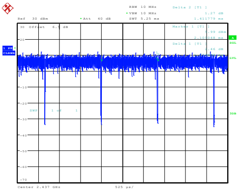
g_2437MHz_Chain 0 1.380ms,1.412ms
