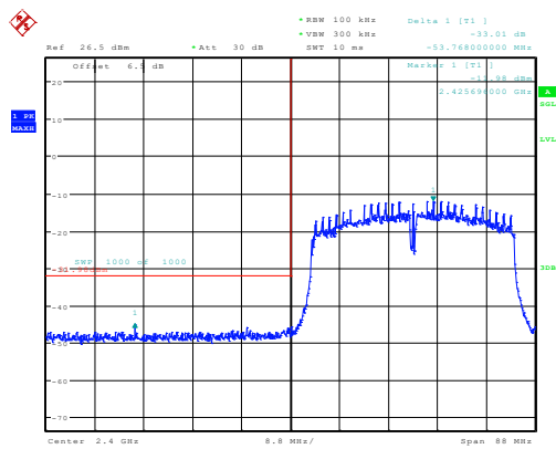
n40_2422MHz_Chain 0 33.01dB
