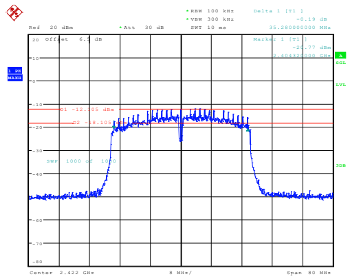
n40_2422MHz_Chain 0 35.280MHz
