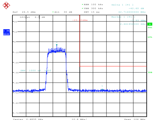
g_2462MHz_Chain 0 42.60dB
