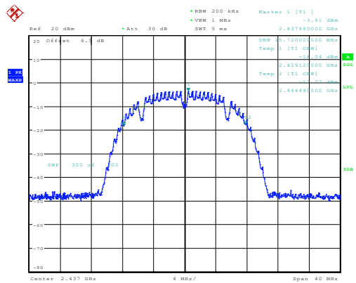
b_2437MHz_Chain 0 15.720MHz
