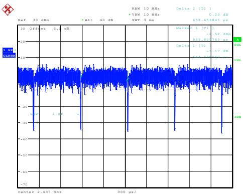
n40_2437MHz_Chain 0 0.644ms,0.659ms
