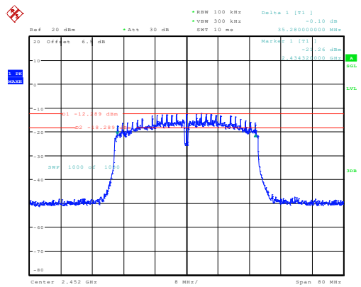
n40_2452MHz_Chain 0 35.280MHz
