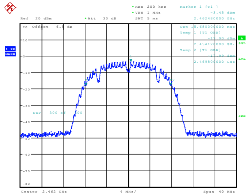
b_2462MHz_Chain 0 15.680MHz
