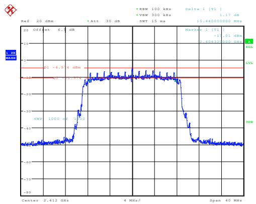
g_2412MHz_Chain 0 15.440MHz
