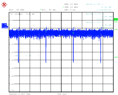
n20_2437MHz_Chain 0 1.292ms,1.316ms
