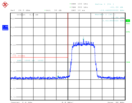
g_2412MHz_Chain 0 41.30dB
