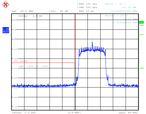
n20_2412MHz_Chain 0 41.10dB
