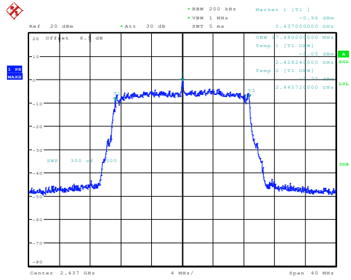
g_2437MHz_Chain 0 17.480MHz
