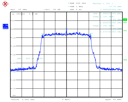
g_2462MHz_Chain 0 17.480MHz
