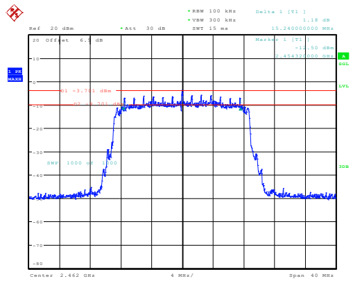
g_2462MHz_Chain 0 15.240MHz
