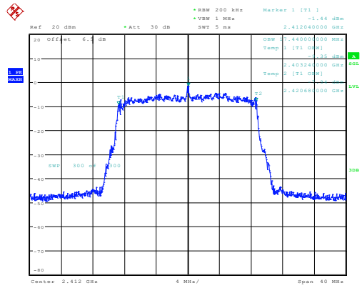
g_2412MHz_Chain 0 17.440MHz
