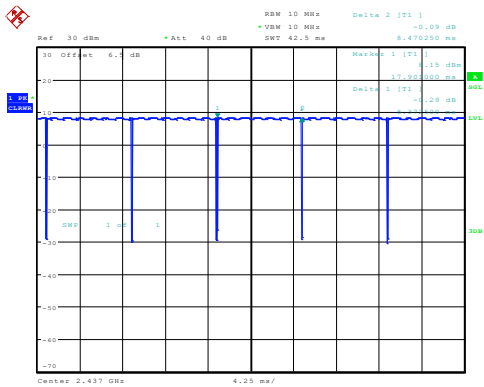
b_2437MHz_Chain 0 8.373ms,8.470ms
