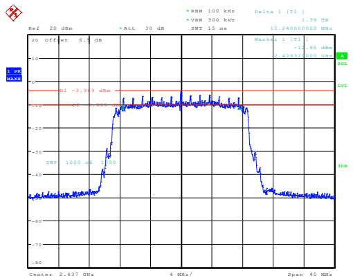
g_2437MHz_Chain 0 15.240MHz
