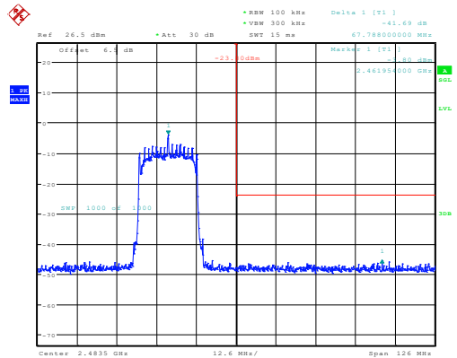
n20_2462MHz_Chain 0 41.69dB
