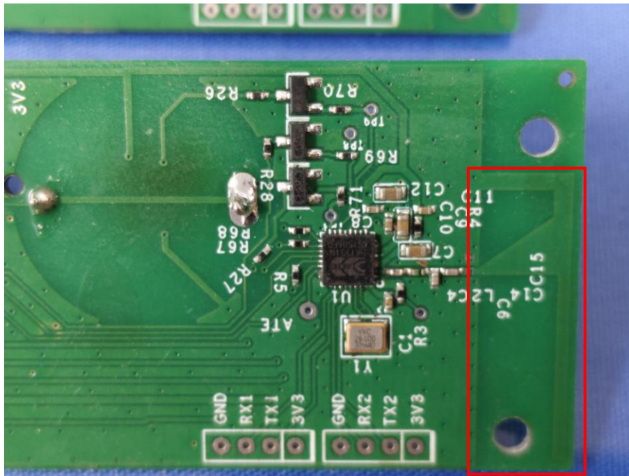
M/N: MTM-200P-15TS-WiFi: Chip and ANT
