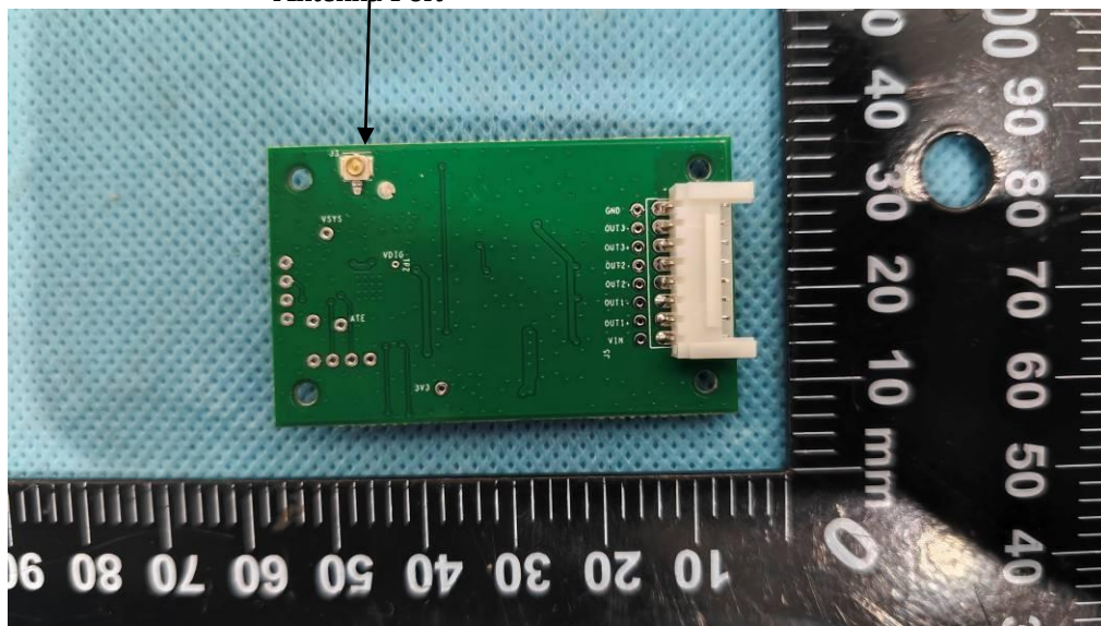
Antenna Port
