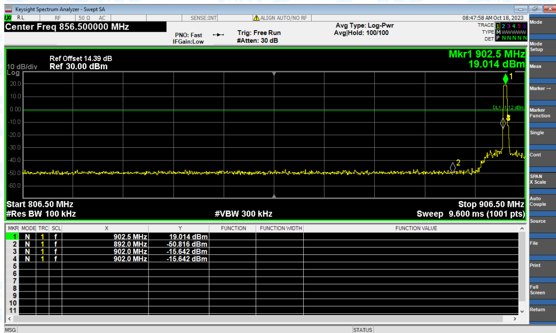
Band Edge NVNT LoRa 902.5MHz Ant1 Emission
