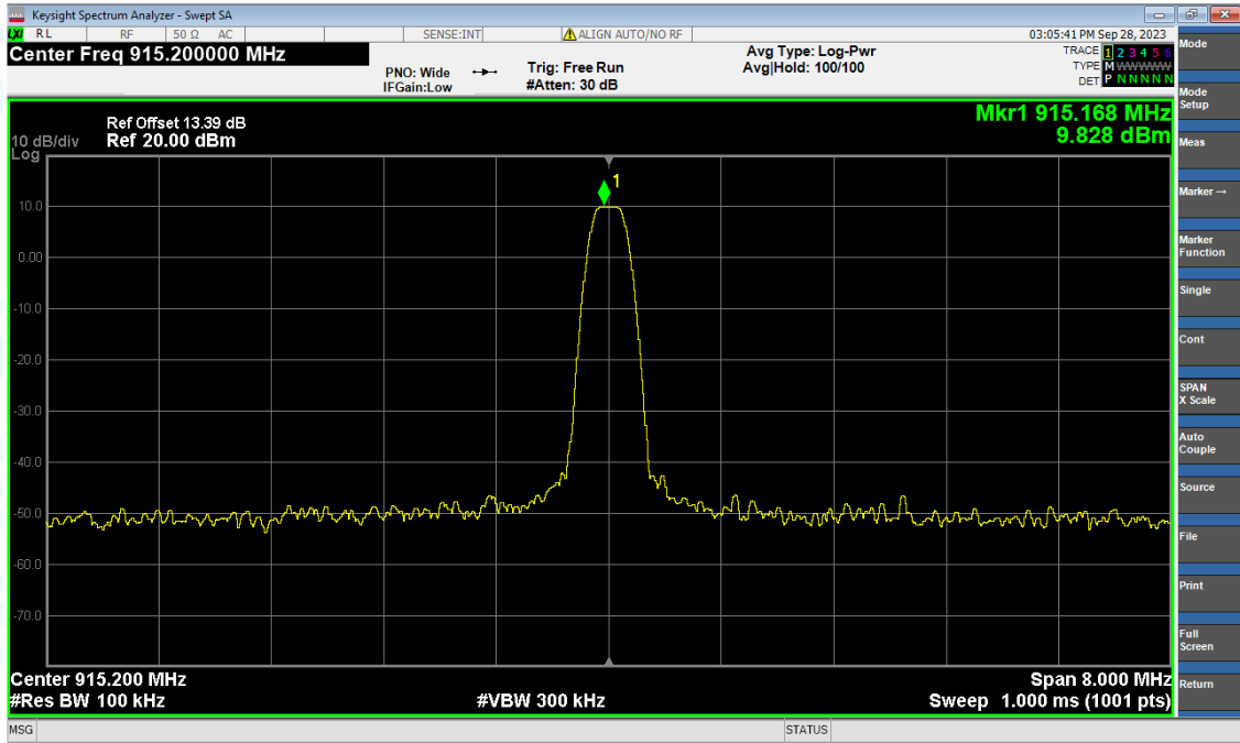
Band Edge NVNT LoRa 915.2MHz Ant1 Emission
