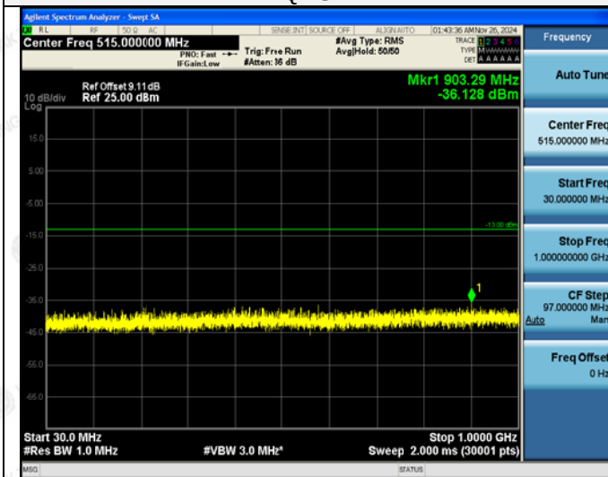
30MHz~1GHz
