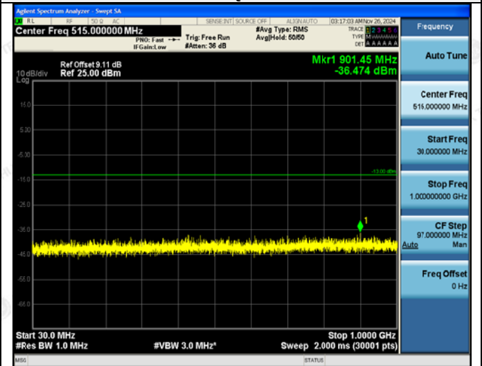
30MHz~1GHz
