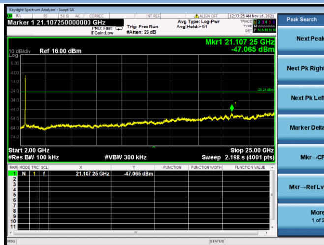
802.11n-40 CHANNEL 8, SPURIOUS 2 GHz ~ 25 GHz
