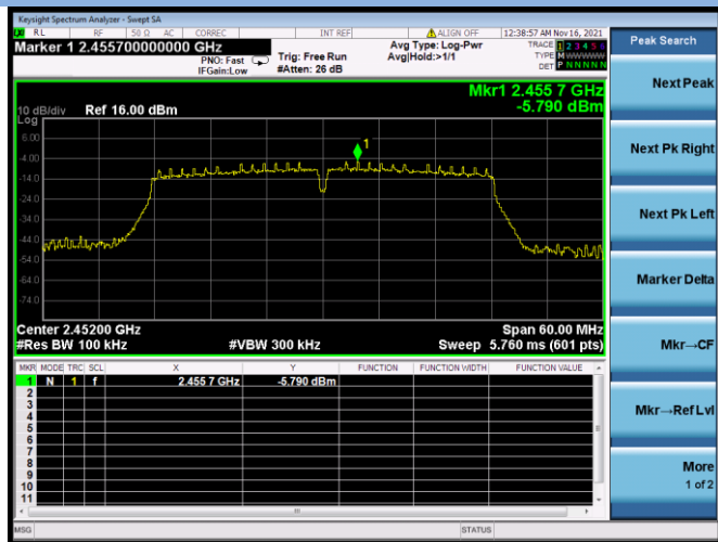
802.11n-40 CHANNEL 9 CARRIER LEVEL
