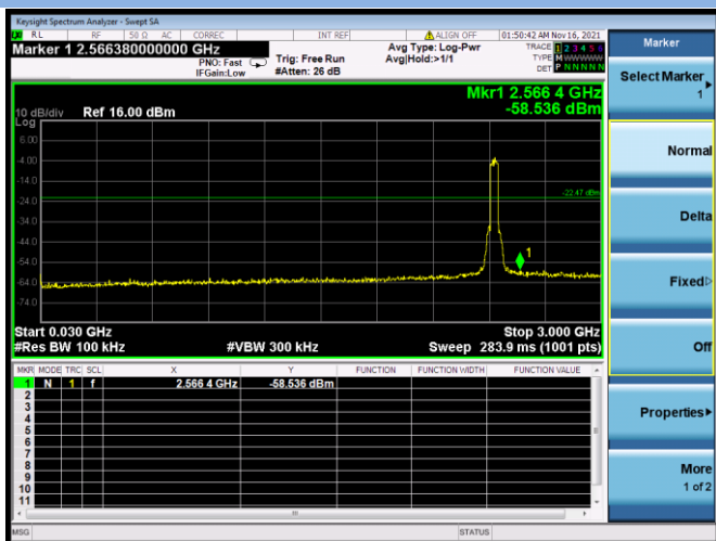
802.11n-40 CHANNEL 5, SPURIOUS 30 MHz ~ 3 GHz
