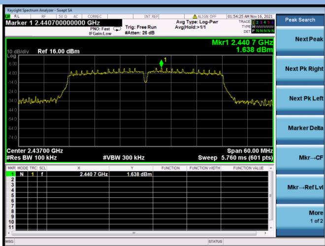
802.11n-40 CHANNEL 6 CARRIER LEVEL
