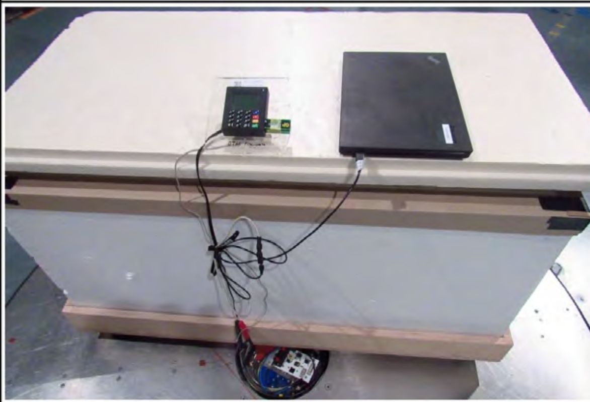
Setup EUT view below 1GHz
