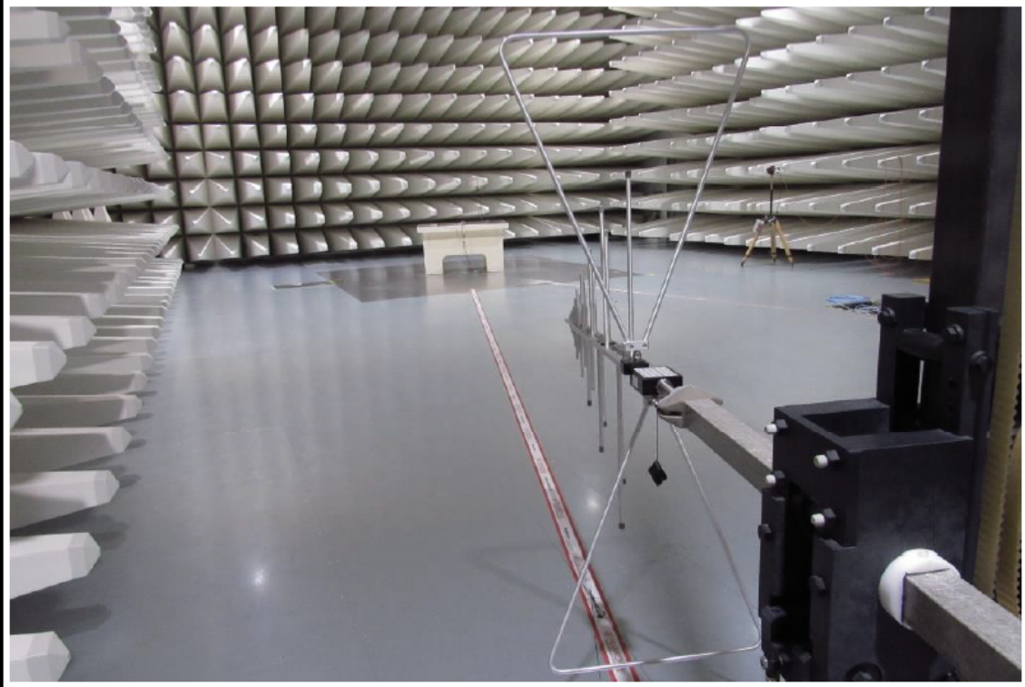
Test setup vertical polarisation
