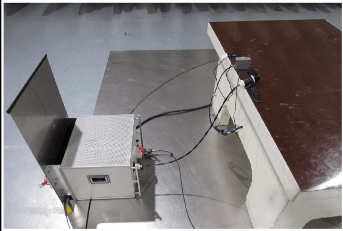
Test setup
