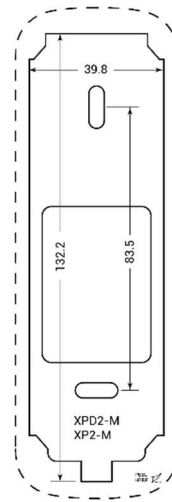
Drilling Template
