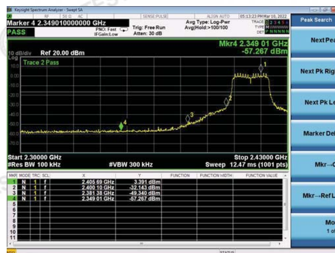
Left bandedge
