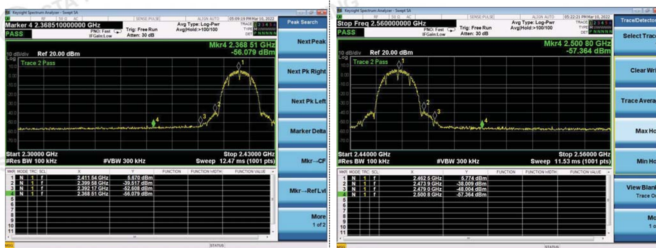
Left bandedge
