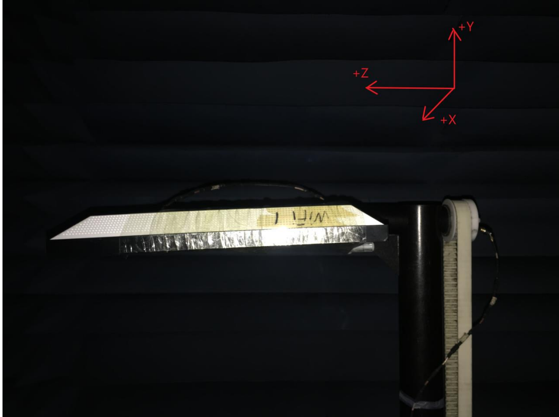
Antenna Gain Setup photo for SY7323
