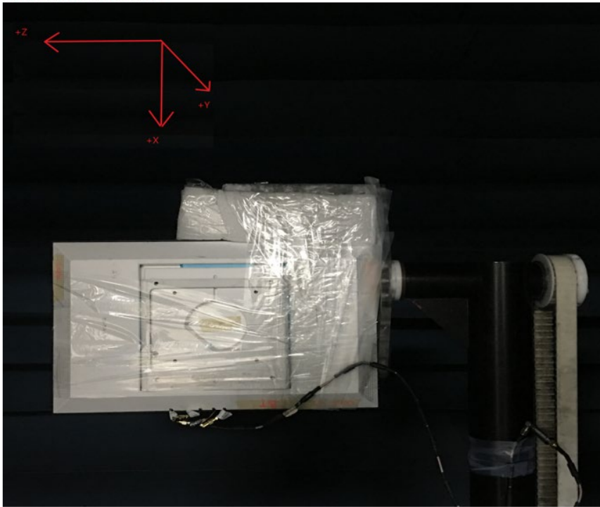
Zigbee_Rotate 90~CW
