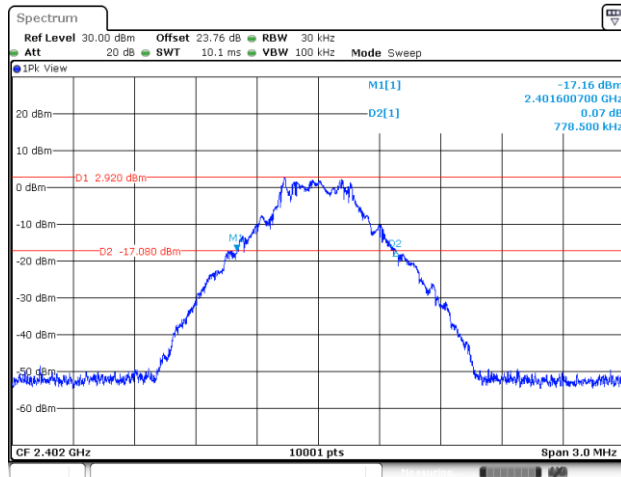
20 dB Bandwidth Plot in Channel 00
