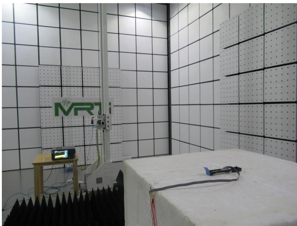
Photograph 3: Set-up photo for Radiated Spurious Emission, 18GHz - 40GHz
