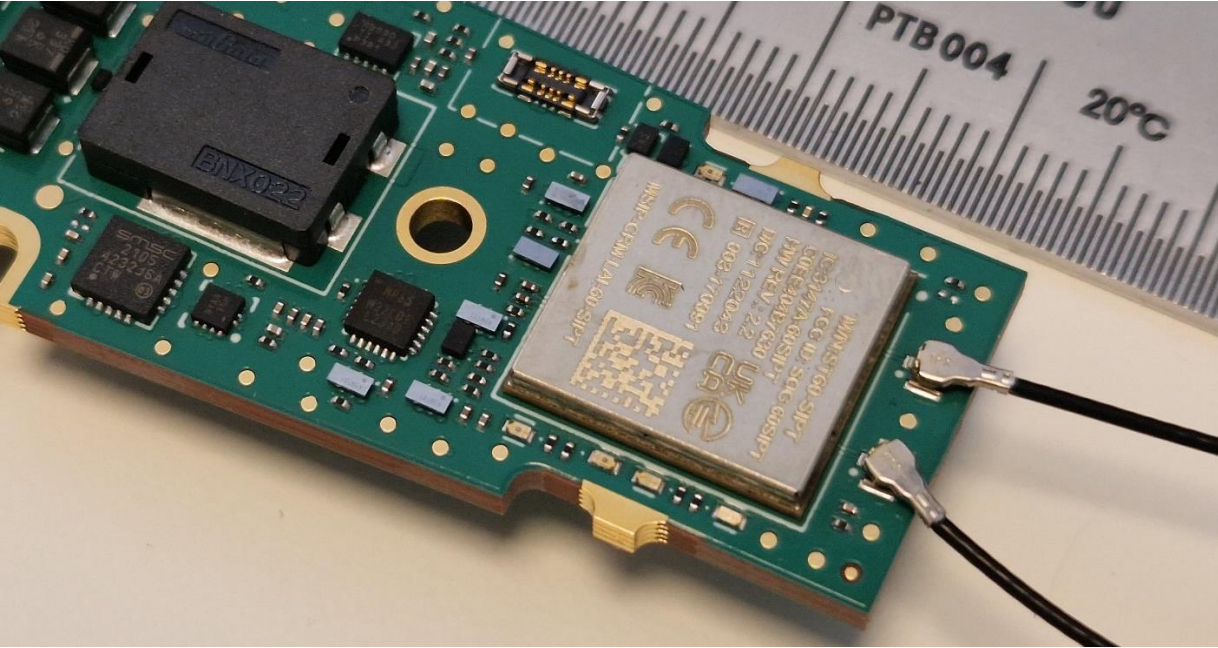
Main PCB bottom
