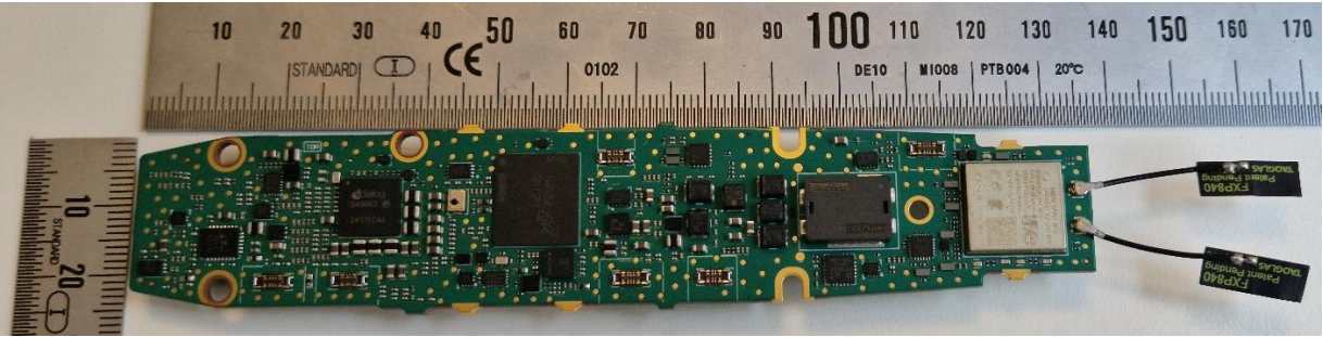
Main PCB top (close-up)
