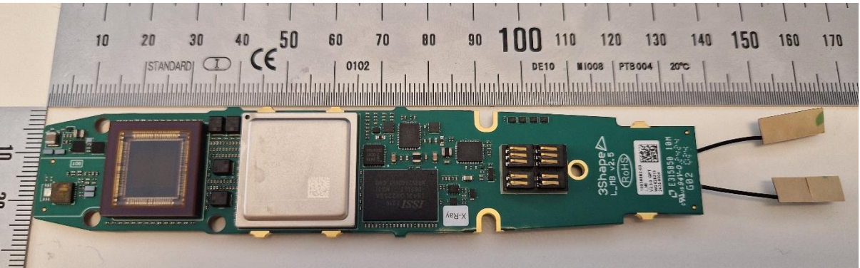
Main PCB bottom
