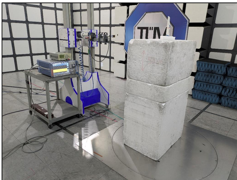
Figure 4 – Radiated Disturbance - 18 GHz to 26 GHz
