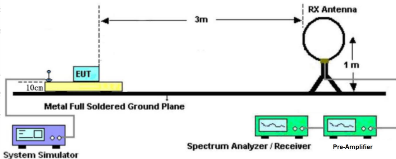
Figure 1. Below 30MHz
