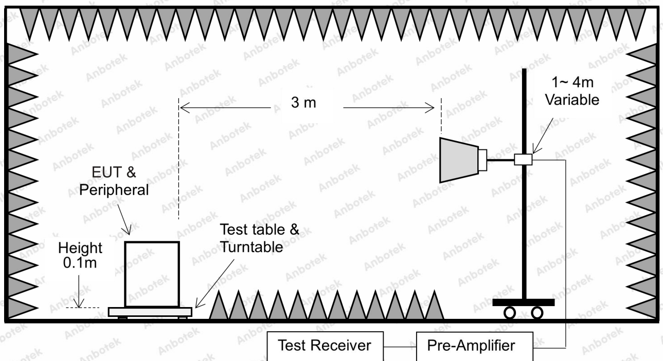
Figure 3. Above 1 GHz
