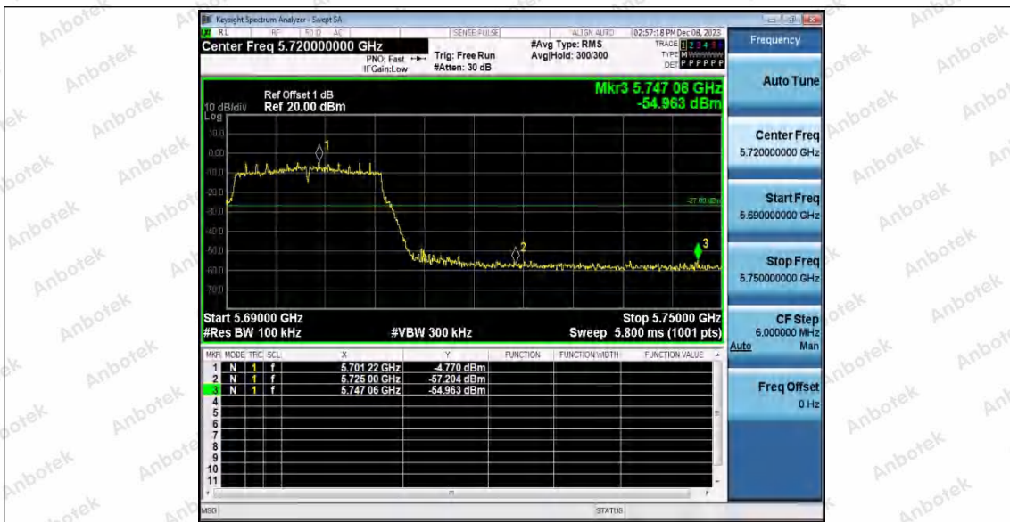
11N20ISO_Ant2_High_5700
