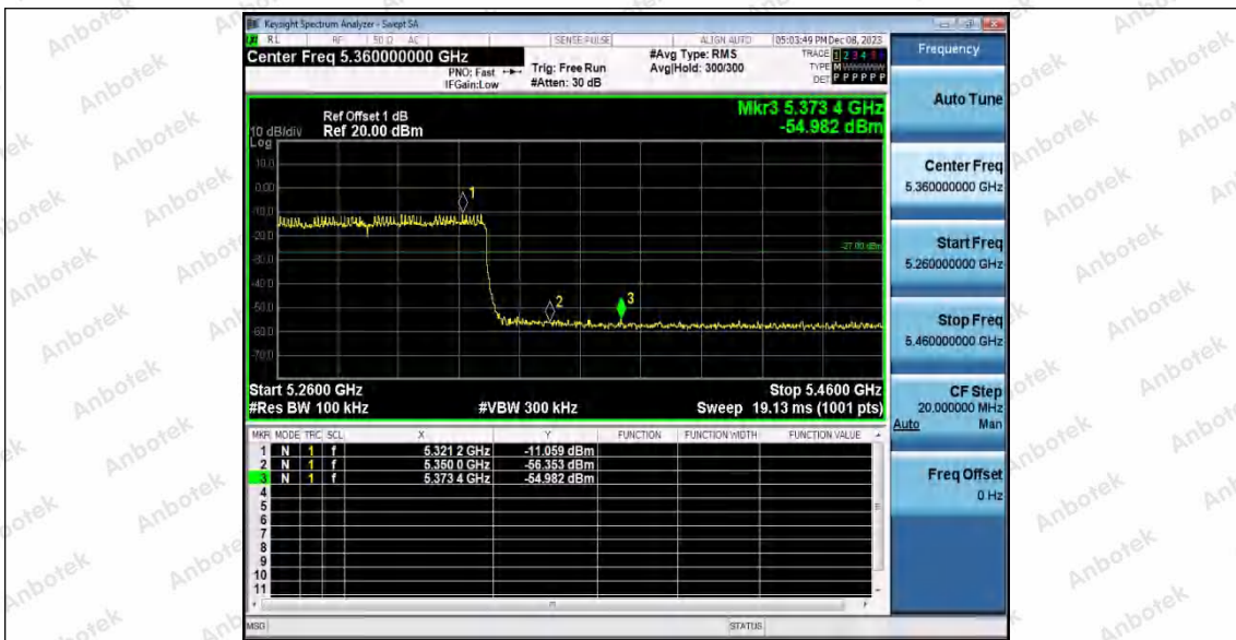
11AX80SISO_Ant2_High_5290
