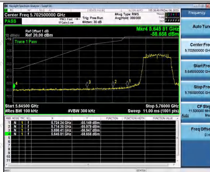
11AX20SISO_Ant1_Low_5745
