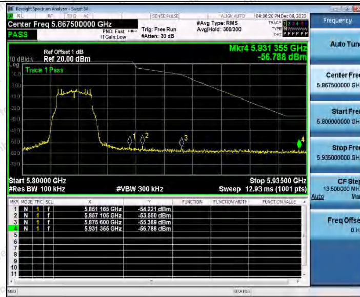
11A_Ant2_High_5825
