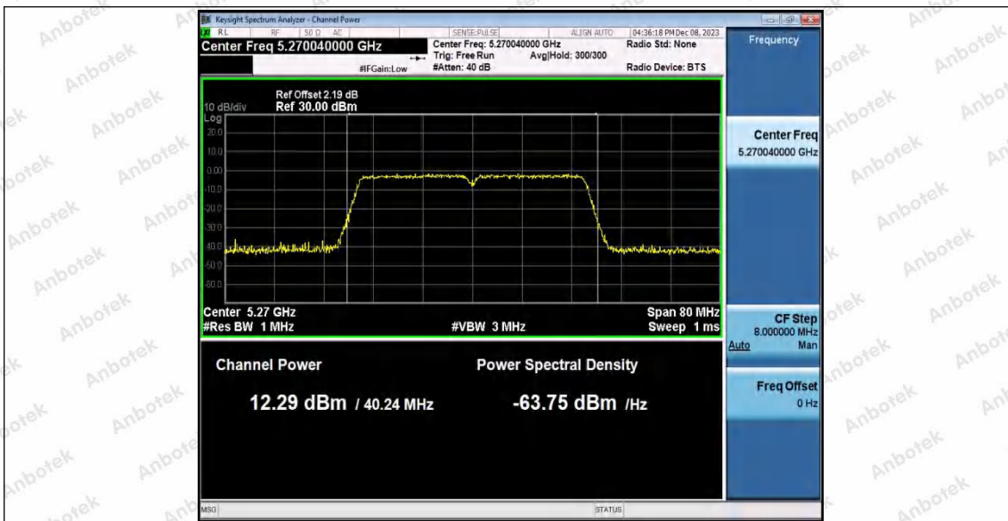
11N40SISO_Ant2_5270
