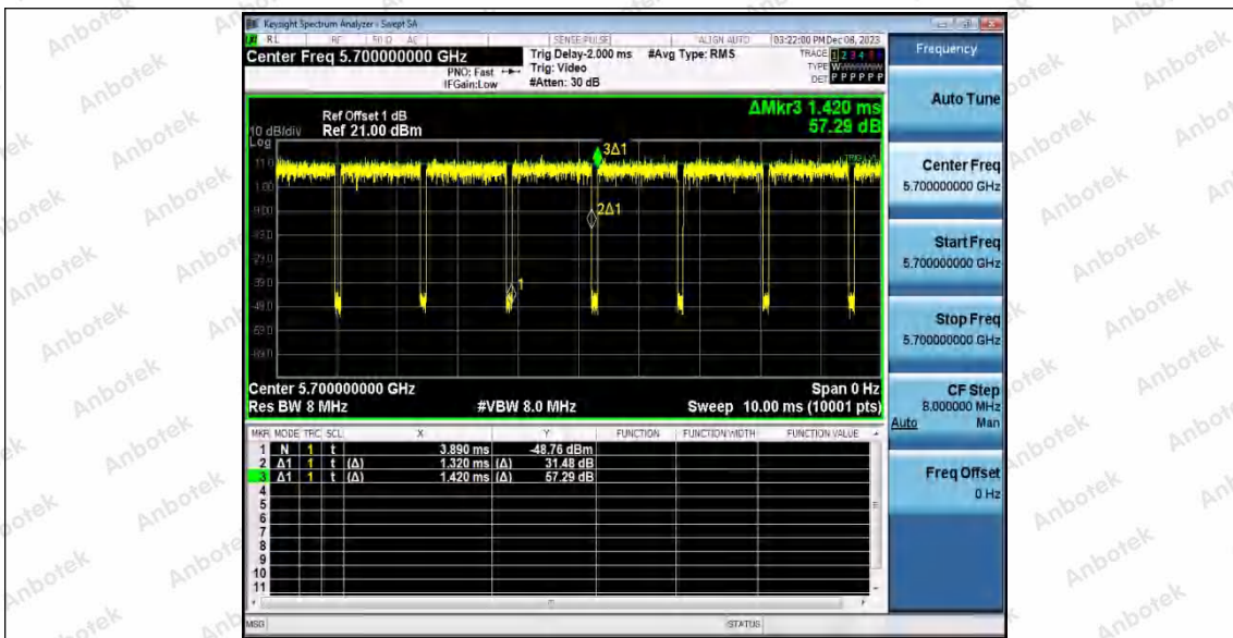
11AC20SISO_Ant2_5700
