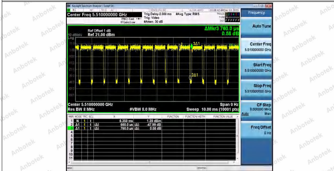
11AC40SISO_Ant2_5510
