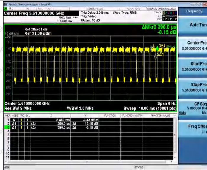
11AX80SISO_Ant2_5610
