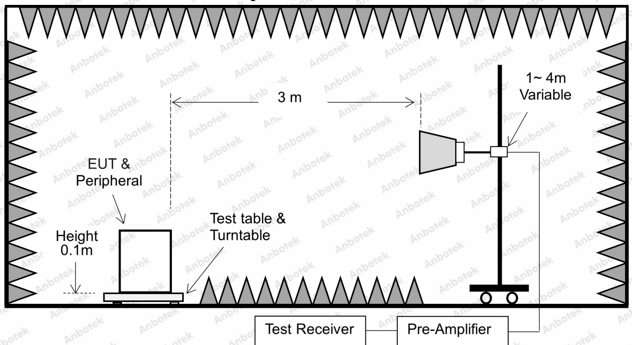
Figure 3. Above 1 GHz
