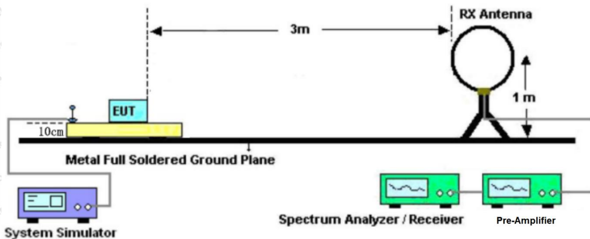
Figure 1. Below 30MHz
