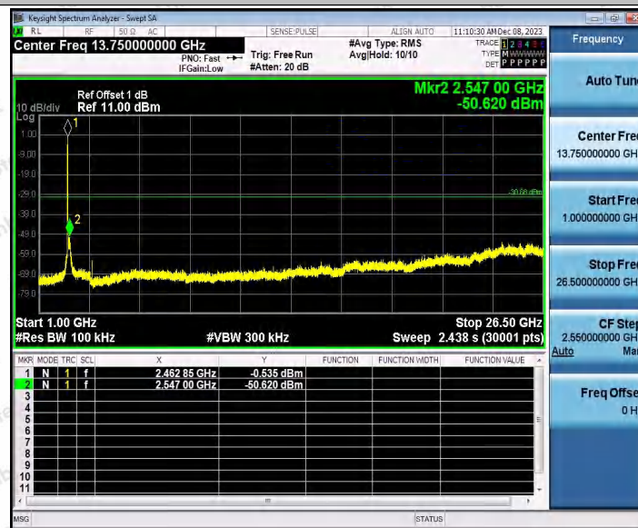
11N20SISO_Ant2_2462_0~Reference
