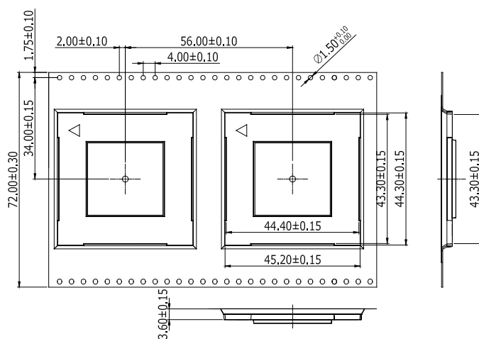
Figure 54: Tape Dimensions
