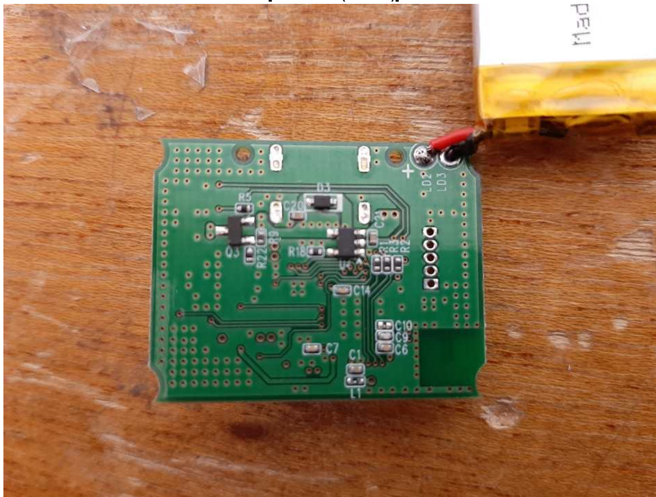
[Main board(Bottom)]
