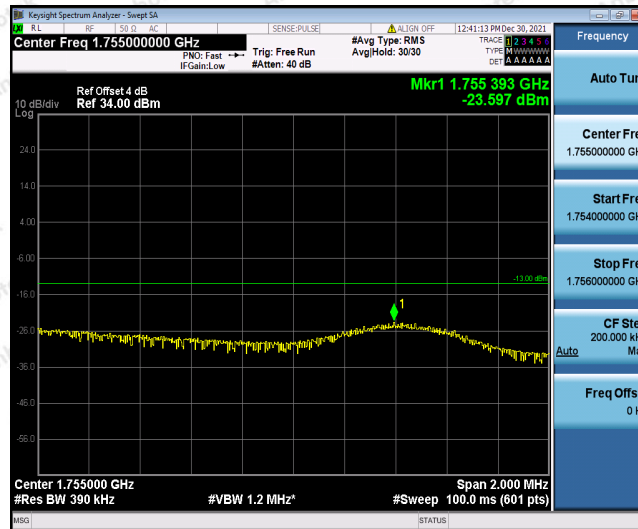
Band4-20MHz-16QAM-20300-1RB#99
