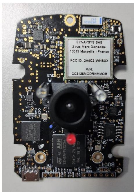
View of the electronic board from (patient's side), with a zoom on the radio module and the antenna
