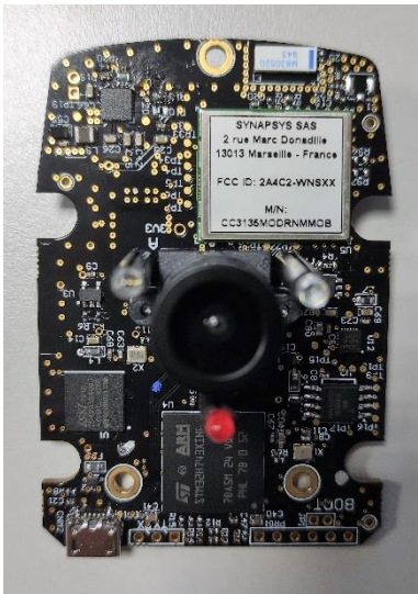
Label applied on the module (left). Board embedding the module mounted (the module cannot be shown, being on the opposite part of the board)
