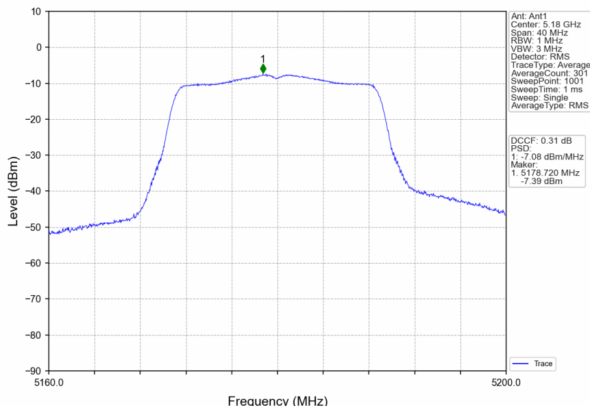
802.11ac(VHT20)_LCH_5180MHz_Ant1_NTNV
