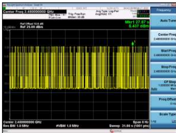
DQPSK,2480,2DH5,Transmission Number
