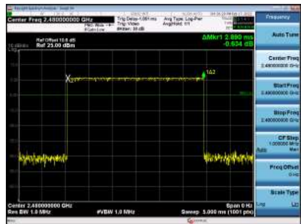
DQPSK,2480,2DH5,Transmission Time
