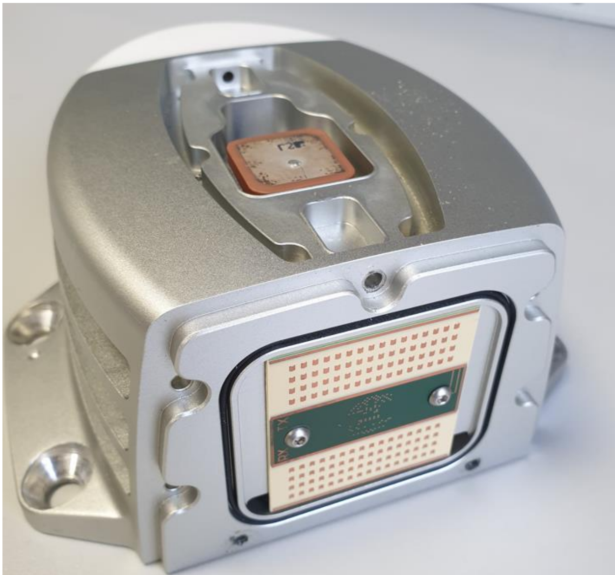
Figure 7 – TN201SP with one RF and the GPS radomes removed
