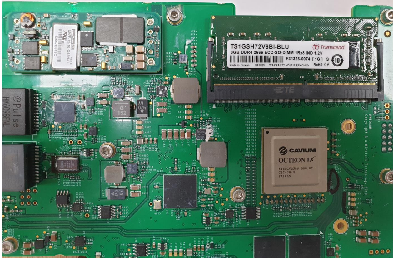
Figure 2 – Inside Back cover of DN201SC showing the BWT050 Network Processor board (BOTTOM)
