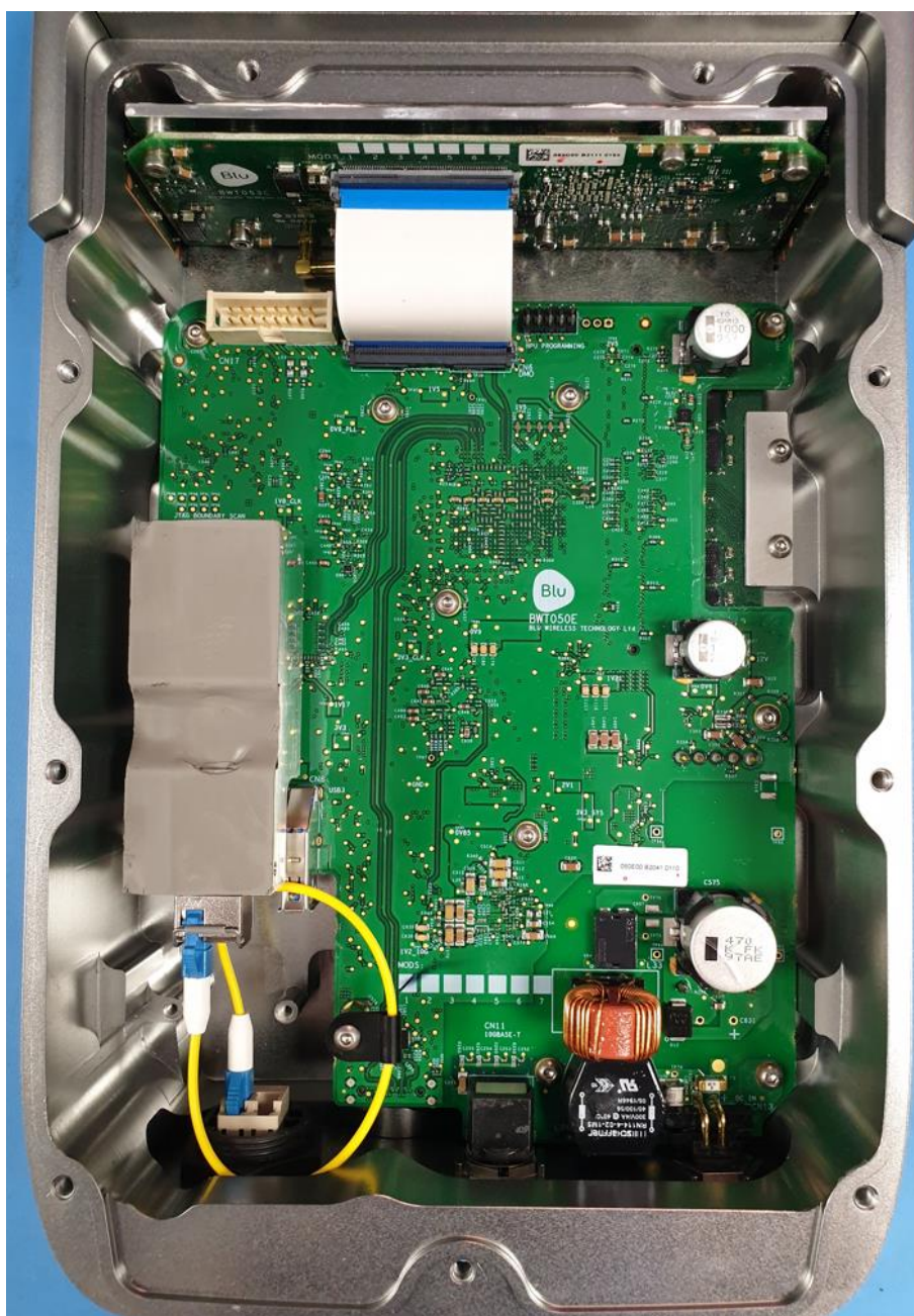
Figure 1 – Inside Back cover of DN201SC showing the BWT050 Network Processor Board (TOP)
