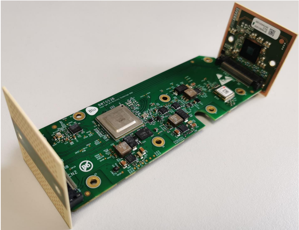
Figure 6 – Representation of both Radio modules connected to BWT053 Modem board
